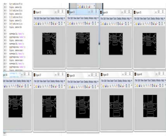
Fig.4.edge detected image
