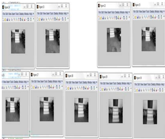
Fig.3.filtered images
